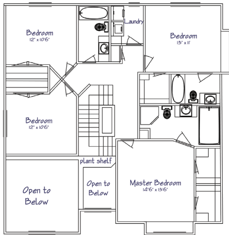
Second Floor: 1154 square feet
